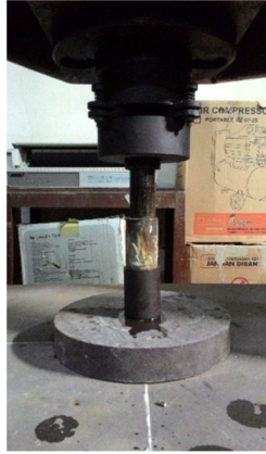
Figure 3. Shear bond strength testing
