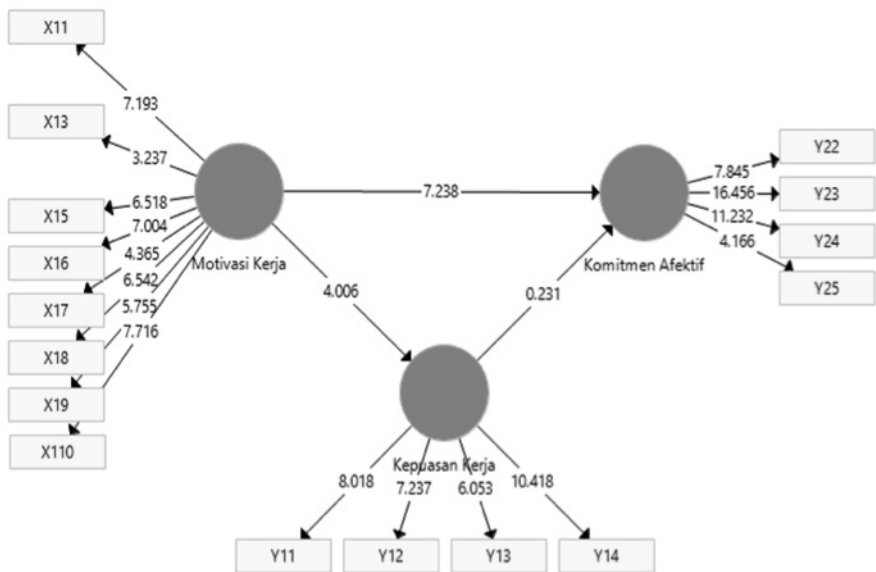
Gambar 2. Hasil Bootstrapping
